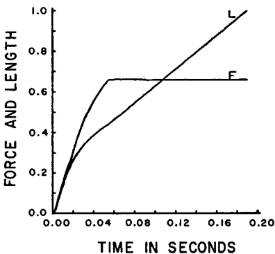
FIGURE 13 The length ( L ) change of the model under a particular force ( F ) constraint computed by using the activation curve labeled "Tetanus" in Fig. 2 (Equation 10). The clamp was applied 54 msec after activation began, when gamma was equal to 1.
